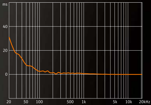
Group Delay
