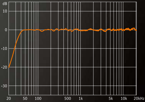
Frequency Response
