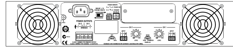
CPS 2.4, CPS 2.6, CPS 2.9 and CPS.12 rear view
