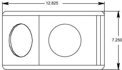
Bose® 203® Loudspeaker Footprint
